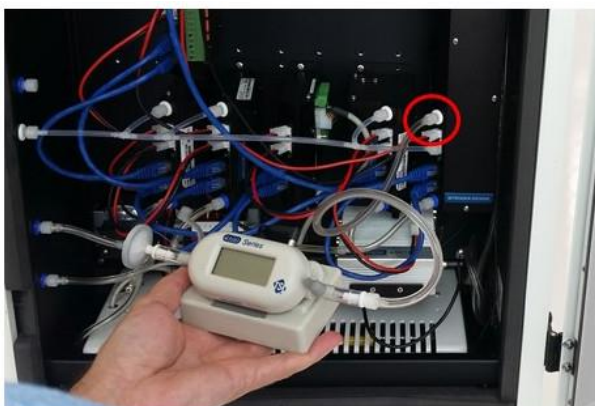
Figure 4-6 To measure the individual module flow rates, disconnect the gas inlet and attach the module inlet to the vacuum port of the R7 flow meter.
