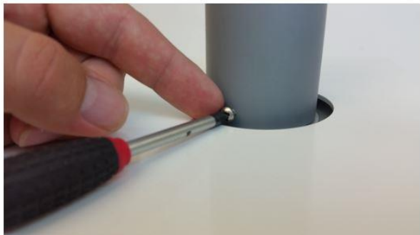
Figure 2-10 During field installation, secure the PM inlet using the retaining screws and plug in the heater
