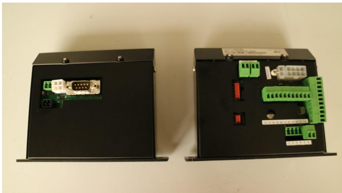
Figure 1-14 Left IO module for the 82850 optical module, note that the fibre span switch is no longer used, Right IO module for the 80180 optical module
