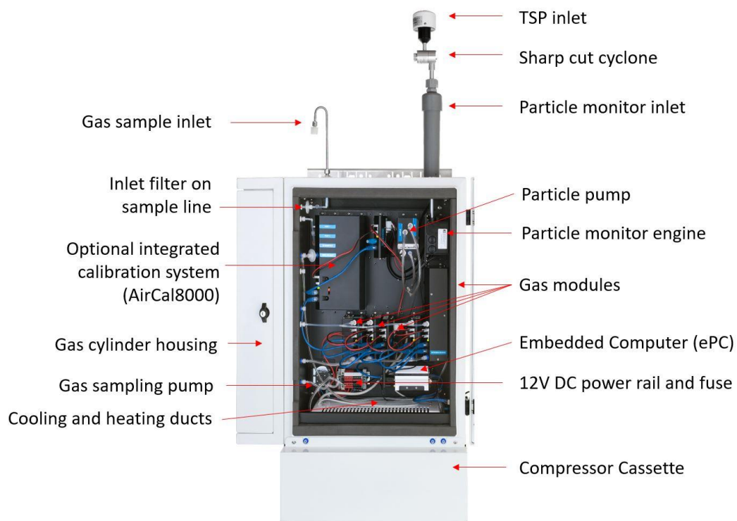
Figure 1-1 AQM 65 with key parts labelled
