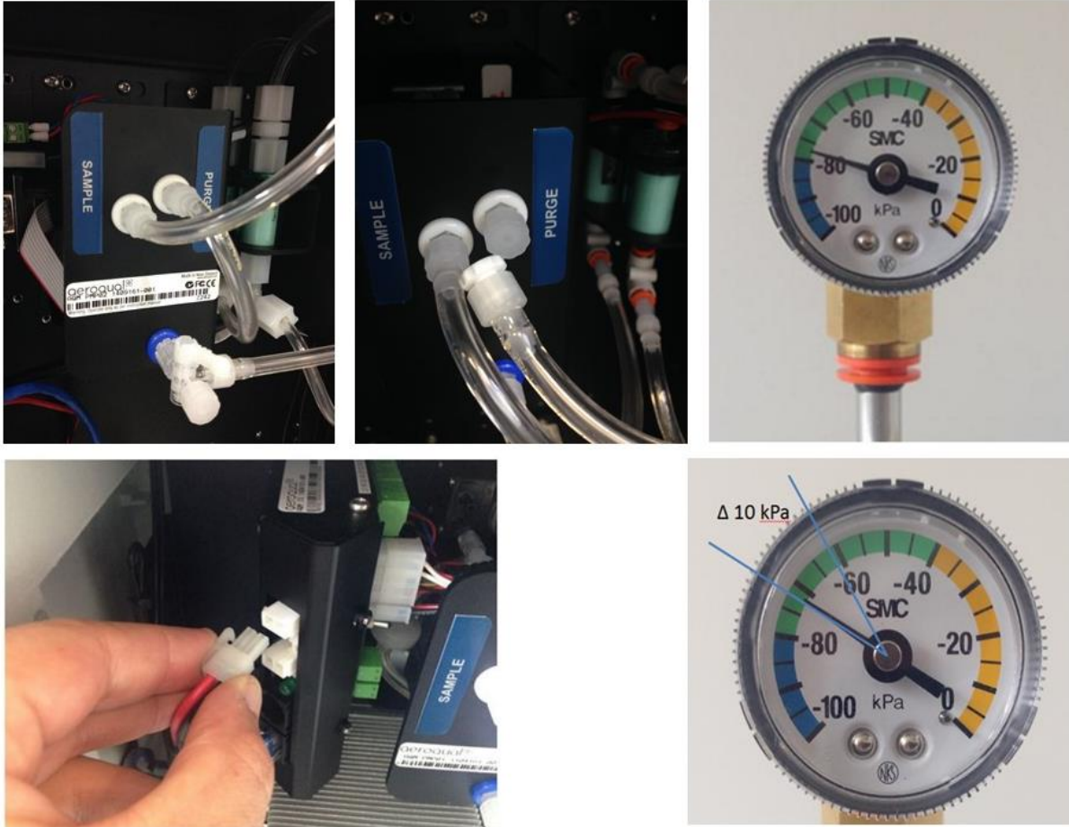
Figure 4-15 Cap the purge and exhaust lines. Place the vacuum gauge on the inlet. Disconnect the power, observe the change in pressure.
