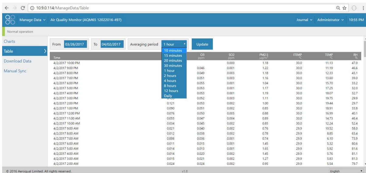
Figure 3-11 The table tool in the Manage Data app shows the data in a table with user configured date range and averaging
