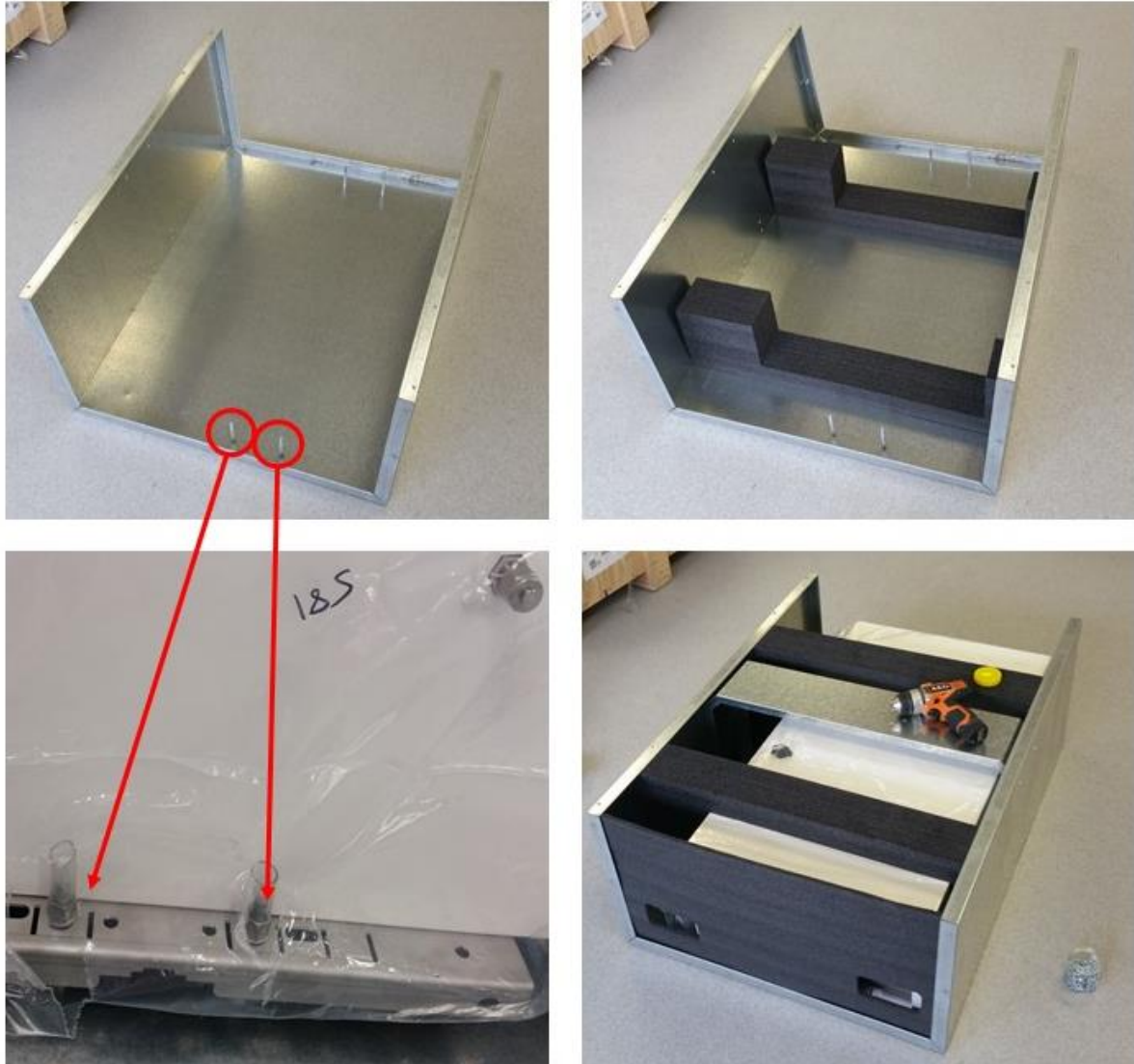
Figure 2-14 The packing crate uses retaining bolts which go through the AQM 65 mounting brackets. There is an additional supporting brace shown in the top right image that should be used.
