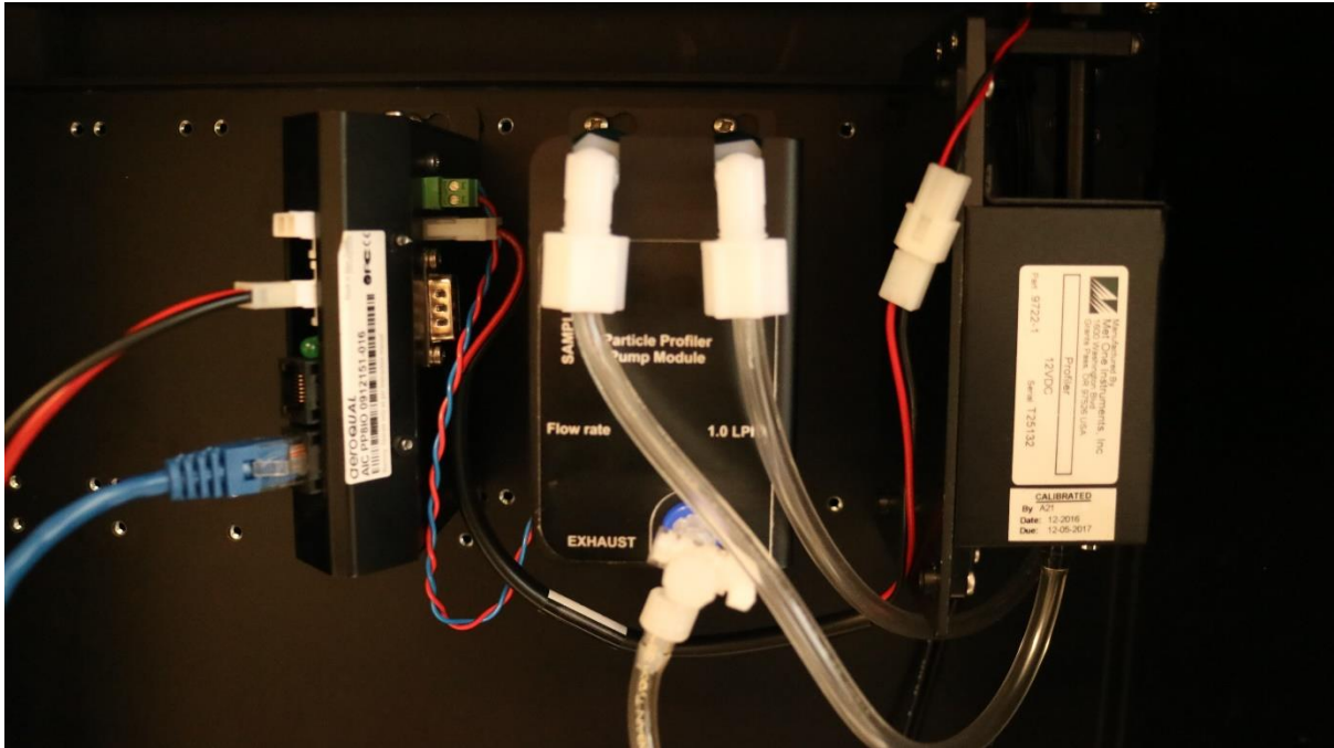
Figure 1-17 An update to the pump module with the filters installed inside the pump module
