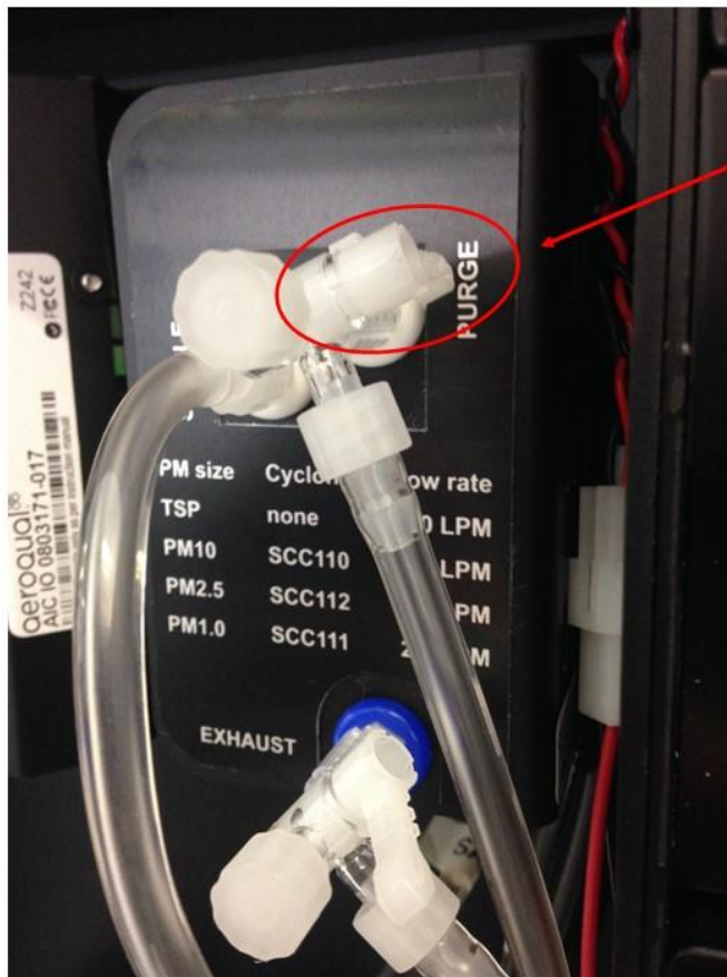
Figure 4-12 The flow rate of the Particle Monitor is set by adjusting the purge and exhaust valves
