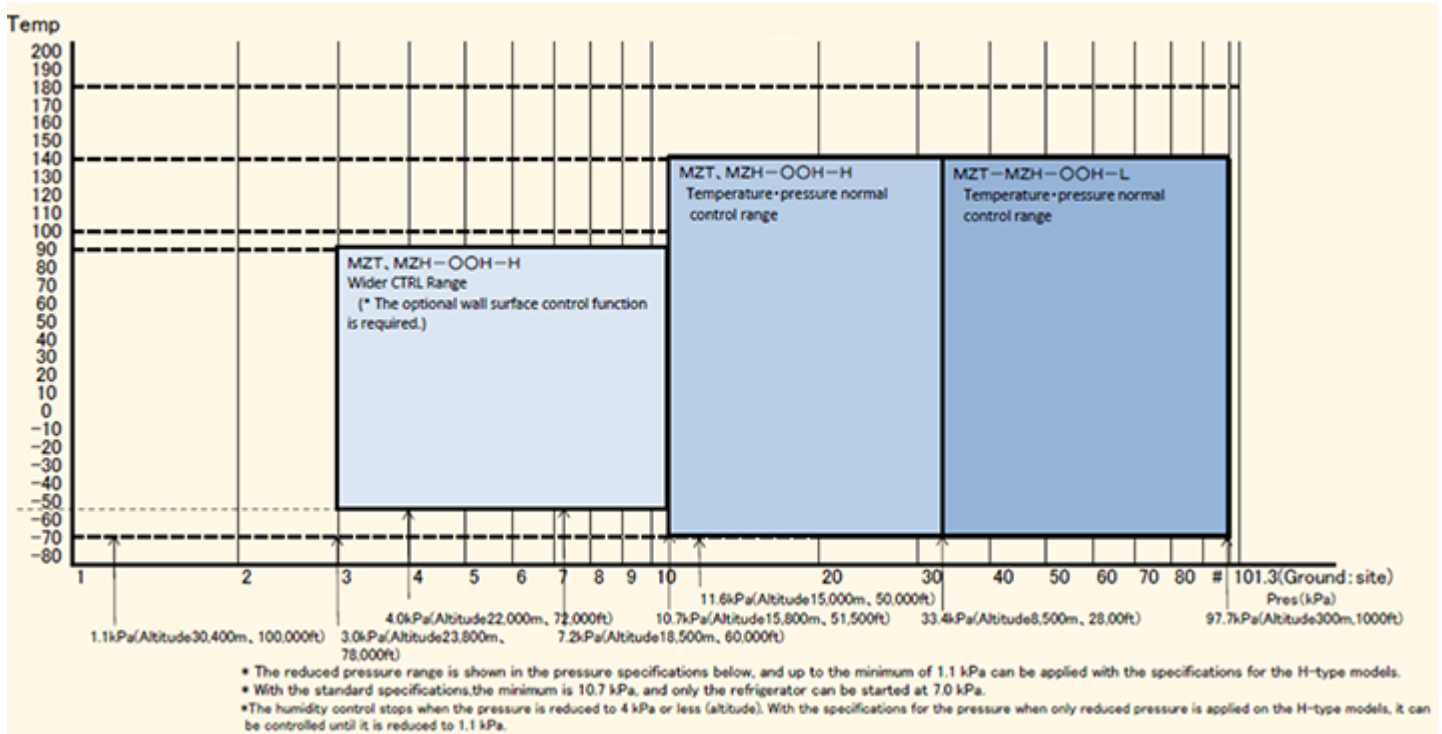
Figure: Pressure/temperature control range of altitude test chamber (MZ Series)
