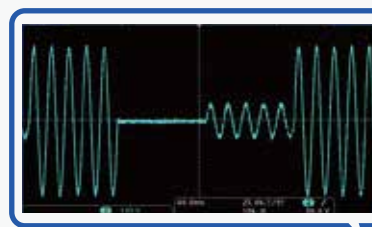
Instantaneous voltage interruption
