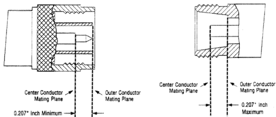
Figure 1 Type-N Connectors
