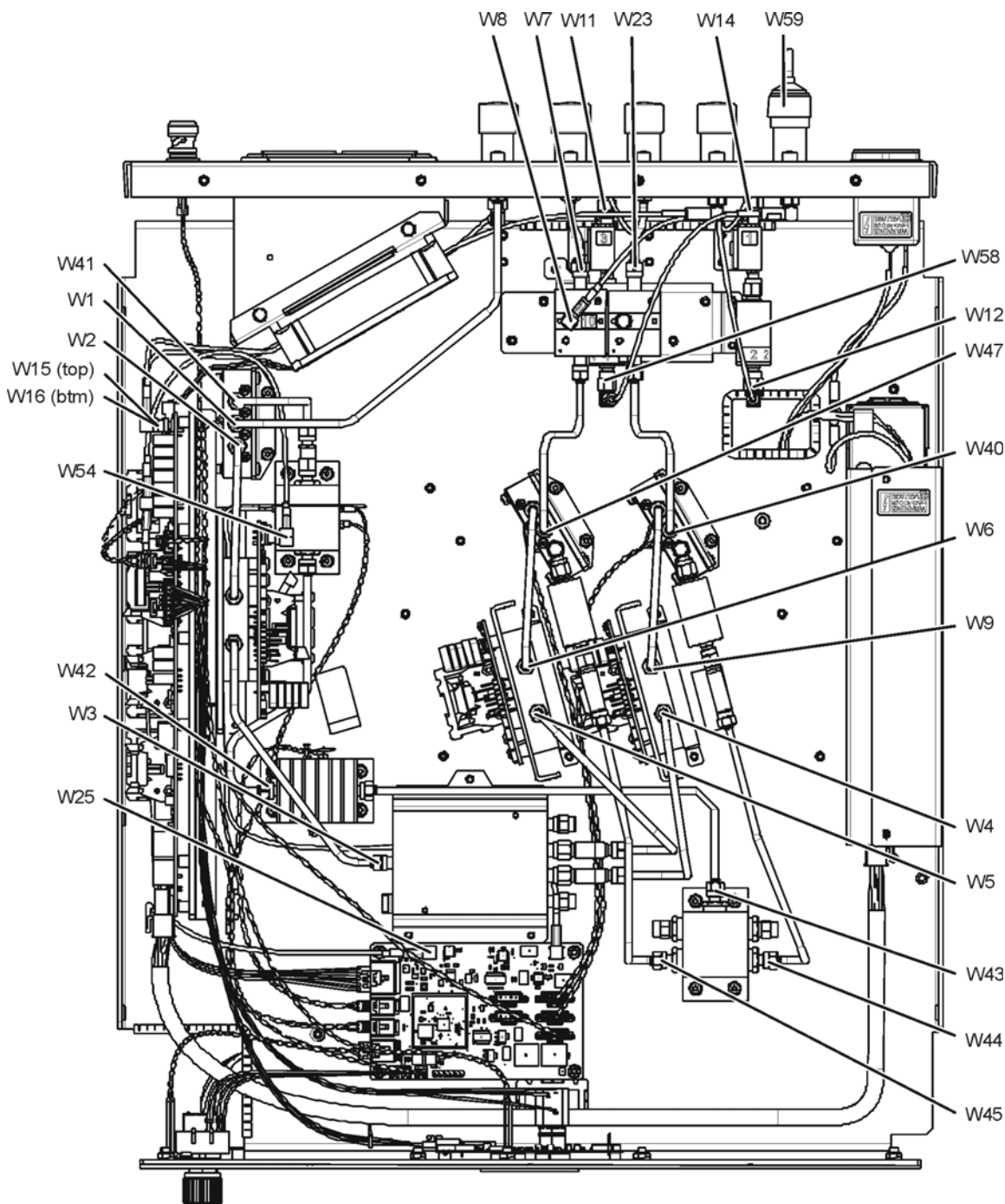
Figure 4-8 Cable Locations (Option 400)
