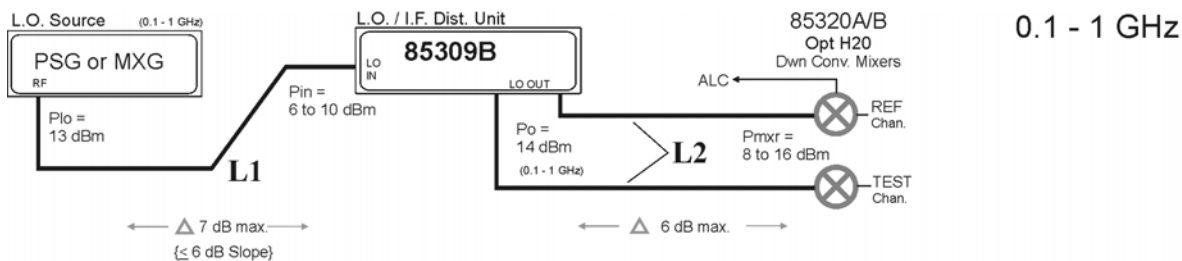
Figure 2-6 Cable Length Configurations (1 of 2)
