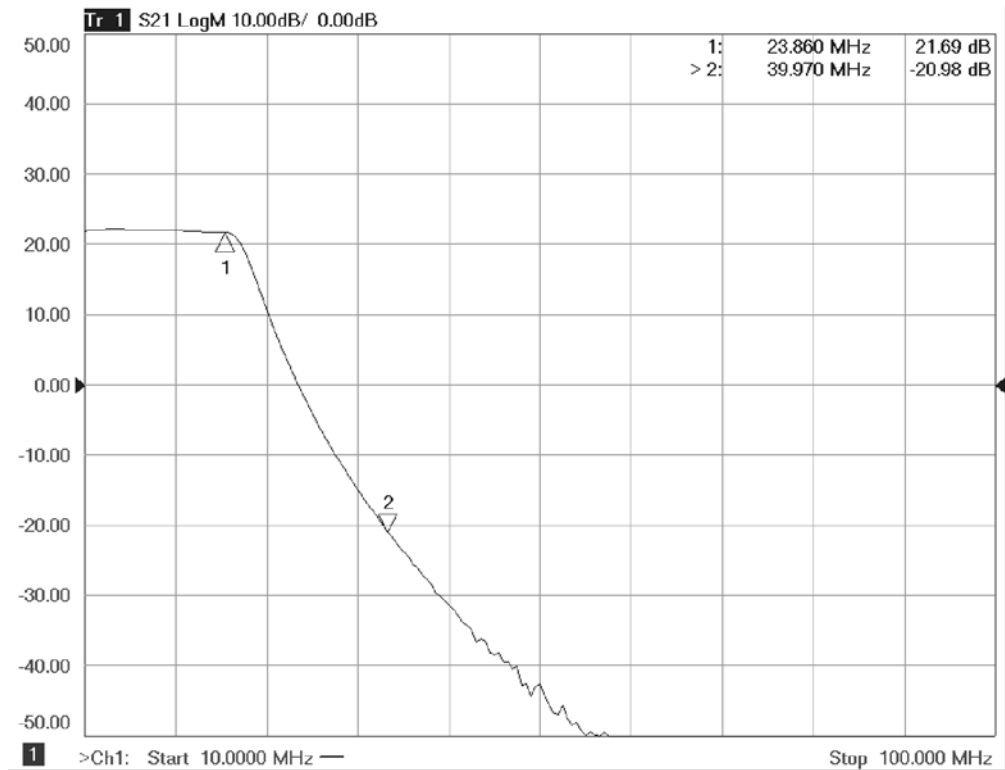
Figure 2-8 Typical IF Gain Response Trace
