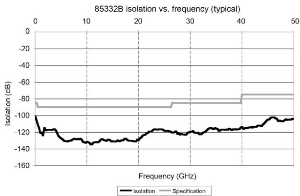
Figure 14. 85332B isolation vs. frequency (typical)
