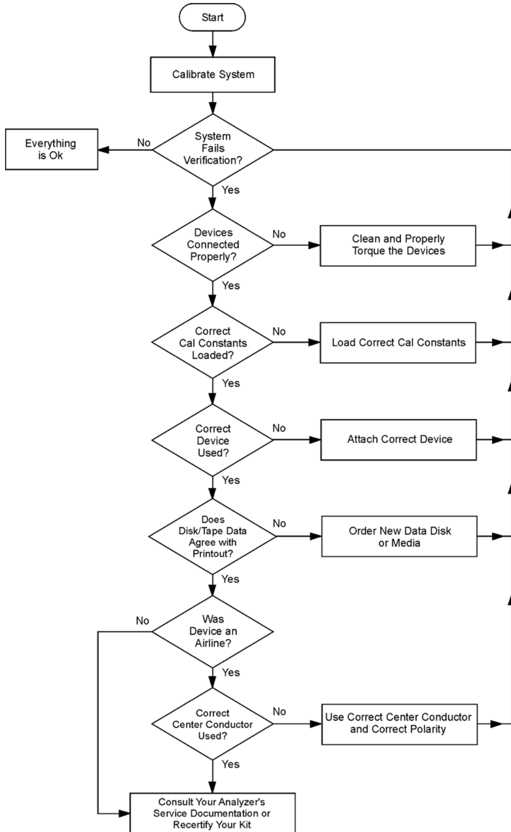
Figure 5-1 Troubleshooting Flowchart
