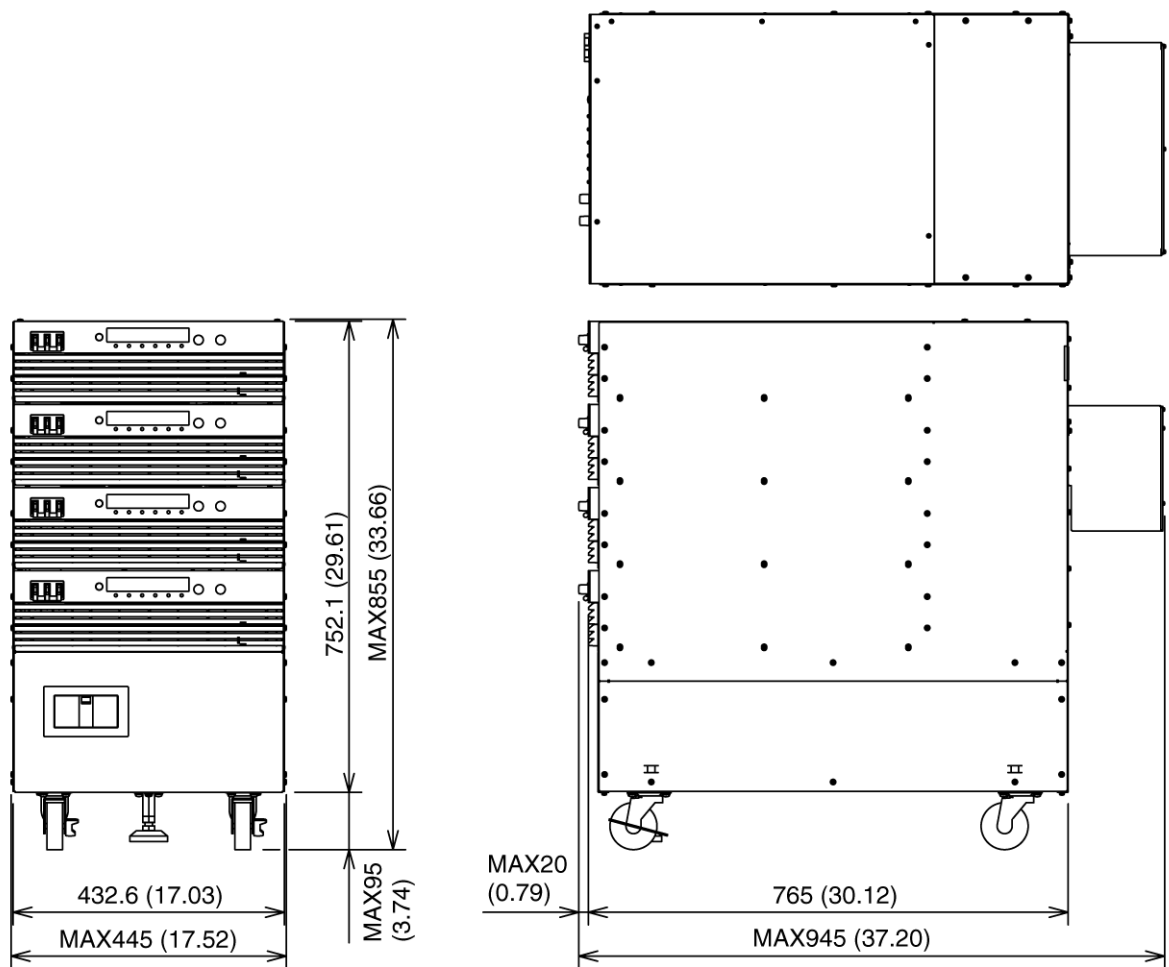
PAT-TMX Series 32 kW System Outline Drawing
