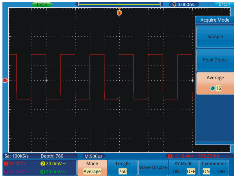
Figure 25. The displayed waveform after the noise is removed under the Average Mode, in which the average number of 16 is set.
