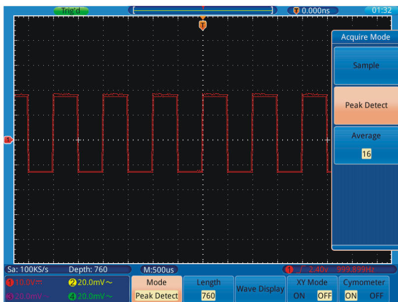
Figure 47. Signal with Noises.
