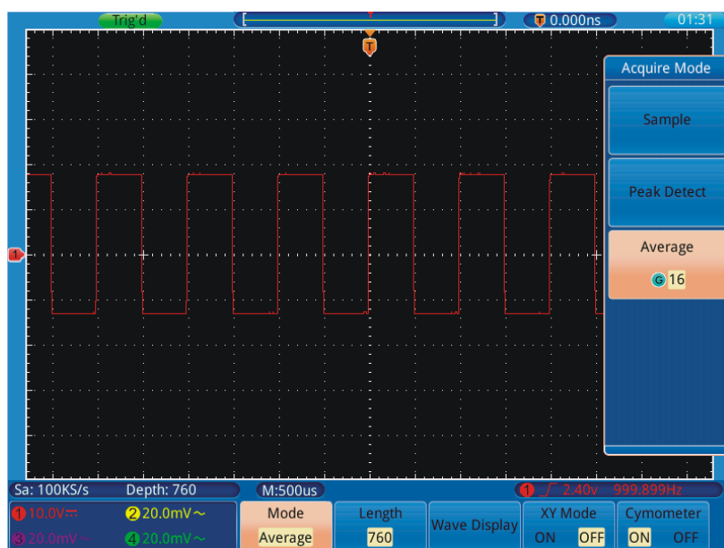
Figure 48. Reduce Noise level by using Average function.
