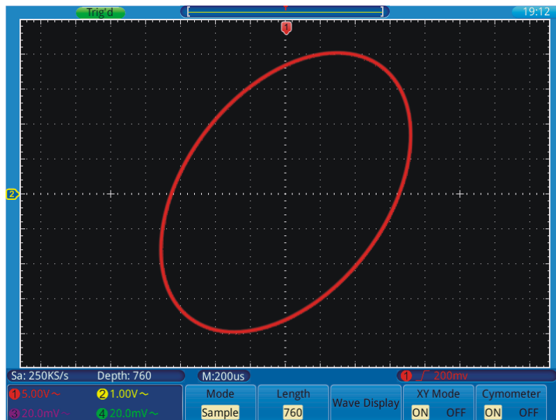
Figure 26. XY Display Mode.
