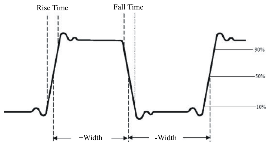
Figure 31. Shows a pulse with some of the time measurement points.
