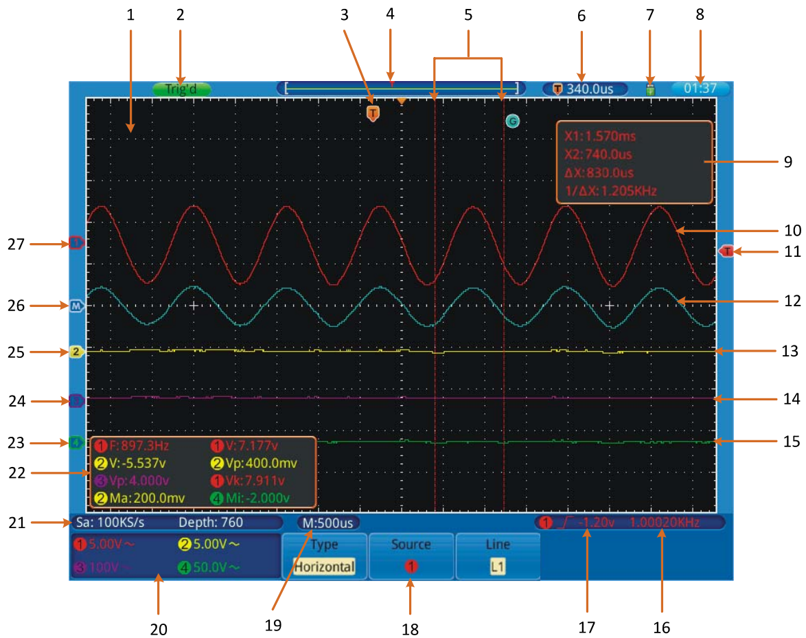
Figure 4. Illustrative Drawing of Display Interfaces.
