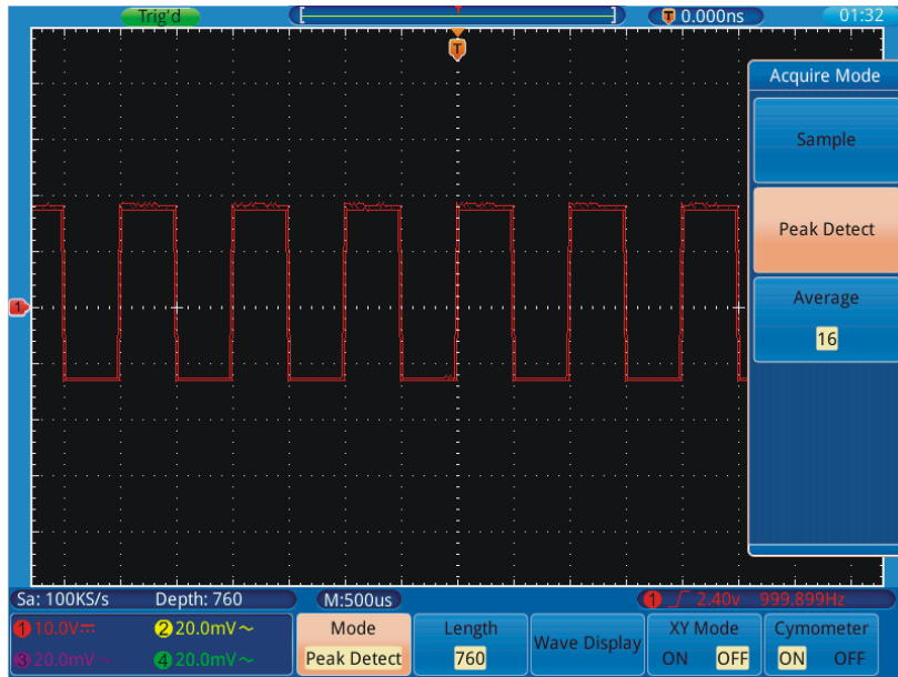
Figure 23. Peak Detect mode, under which the burrs on the falling edge of the square wave, can be detected and the noise is heavy.
