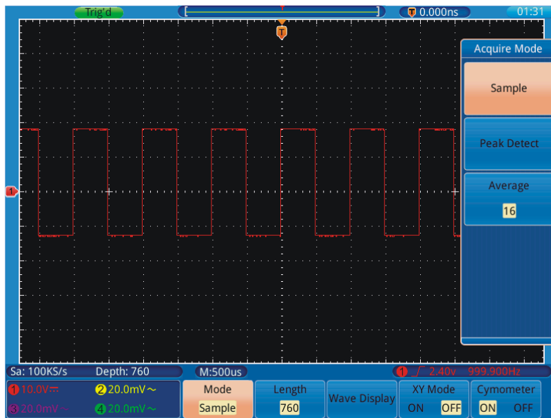
Figure 24. Normal ACQU Mode display, in which no burr can be detected.
