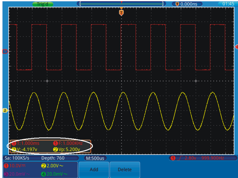
Figure 44. Measure Frequency and PK-PK value for a given signal.
