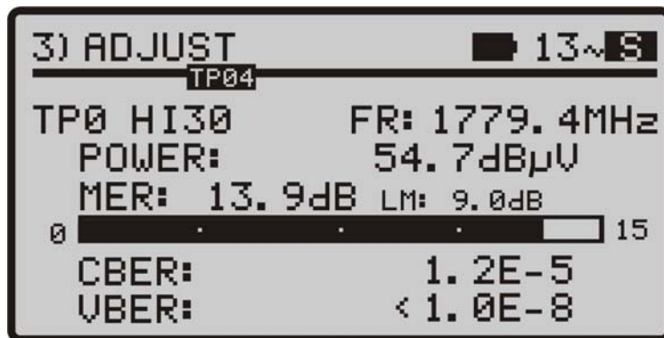
Figure 14.- DVB-S measurements with VBER.
