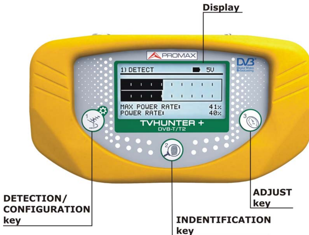
Figure 5. Front panel.
