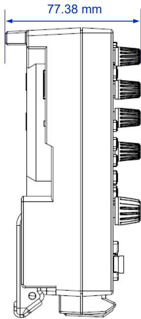
Figure 4.2 Side View
