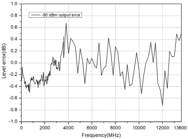
Measured at -90 dBm, level error vs frequency
