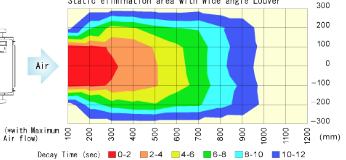
Static elimination area with Wide angle Louver
