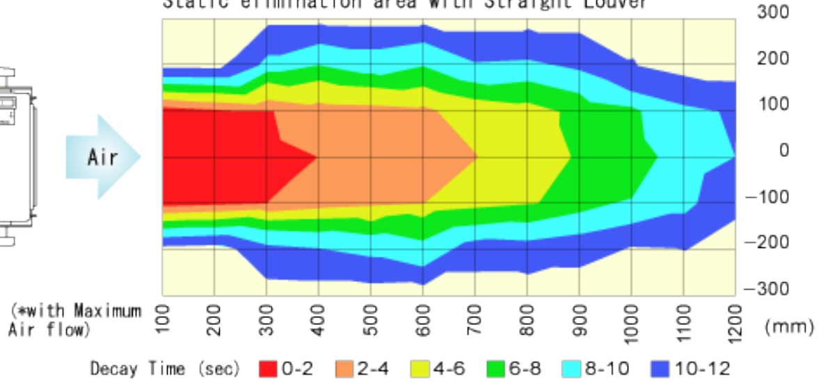
Static elimination area with Straight Louver
