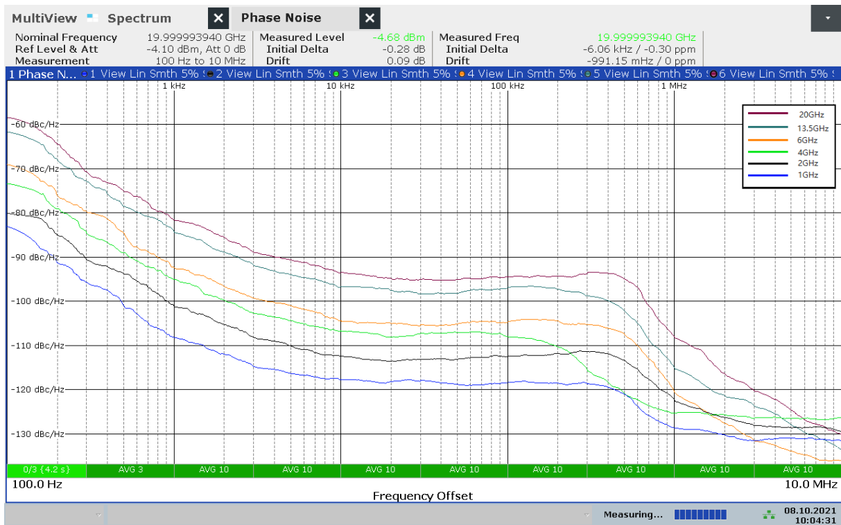
SSB phase noise
