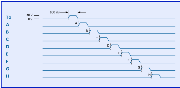
Opt. 02 rear-panel outputs (30 V)
