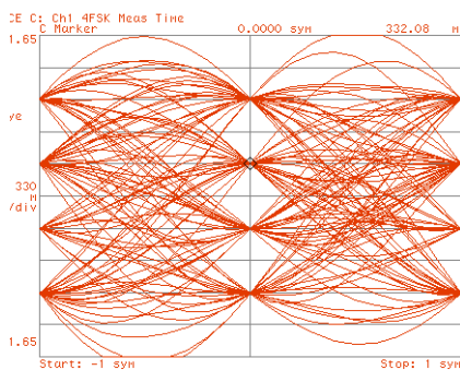
APCO-25 I-Eye diagram (850 MHz carrier)
