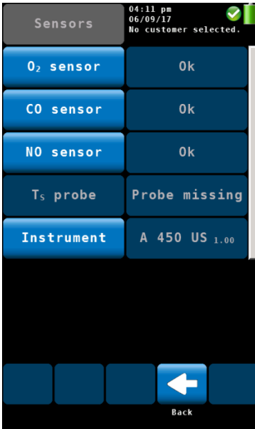
Fig. 42: Sensor diagnosis
